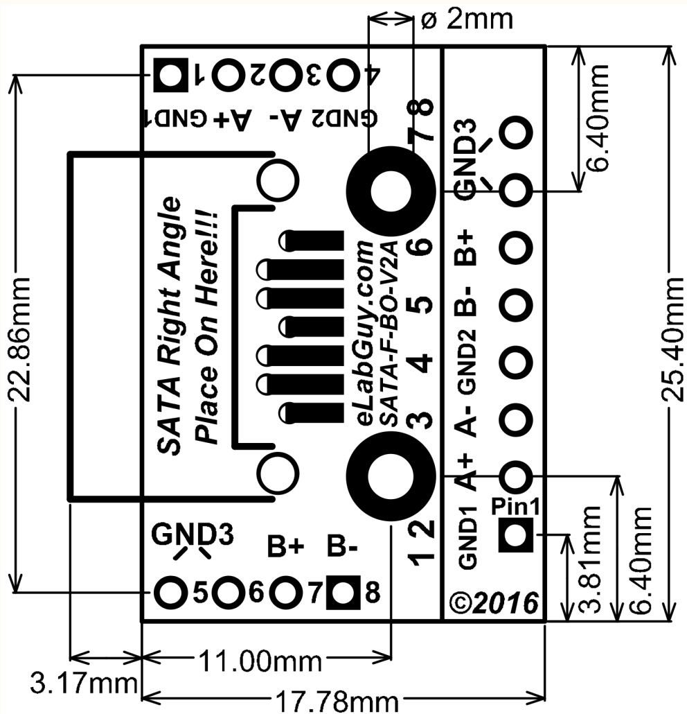
PCB outline Drawing
